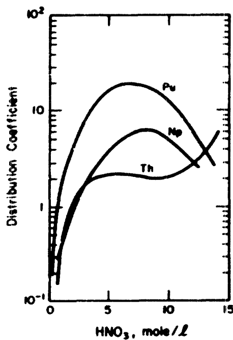
Figure 5. Distribution Coefficients for the Extraction of Tetravalent Actinides by 19 vol % TBP-Kerosene from Nitric Acid Solution. 165
