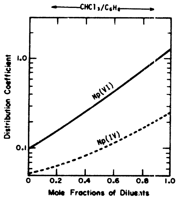
Figure 16. Neptunium Extraction with TBP from 5M HNO 3 into Diluent Mixtures. 203
