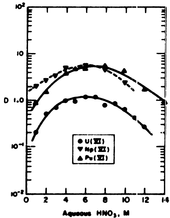
Figure 12. The Extraction of the Hexavalent Actinide Nitrates by 10 vol % TOA in Xylene. 190
